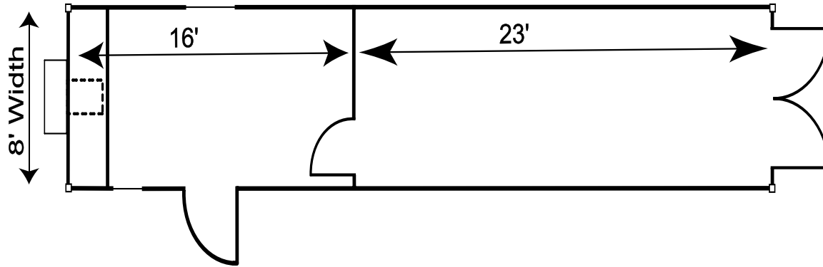
40' Ground Level Office and Storage Container
